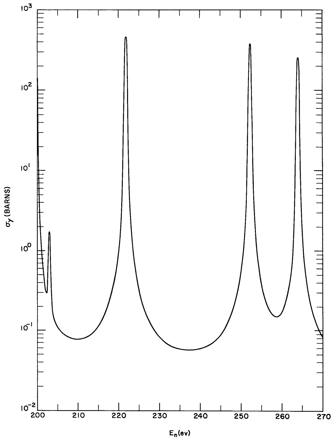
Fig. 6 Thorium-232 radiative capture cross section, \sigma_\gamma , versus neutron energy, E_n , from 200 to 270 ev for T = 0.0253 ev.
