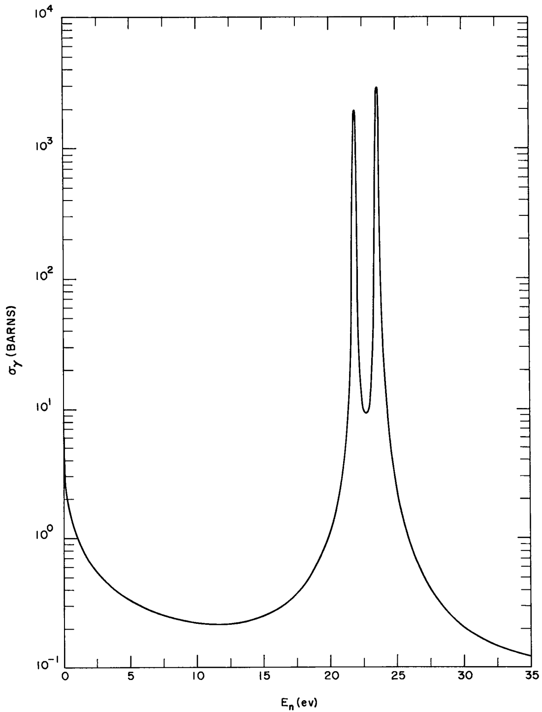
Fig. 2. Thorium-232 radiative capture cross section, \sigma_\gamma , versus neutron energy, E_n , from 0 to 35 ev for T = 0.0253 ev.
