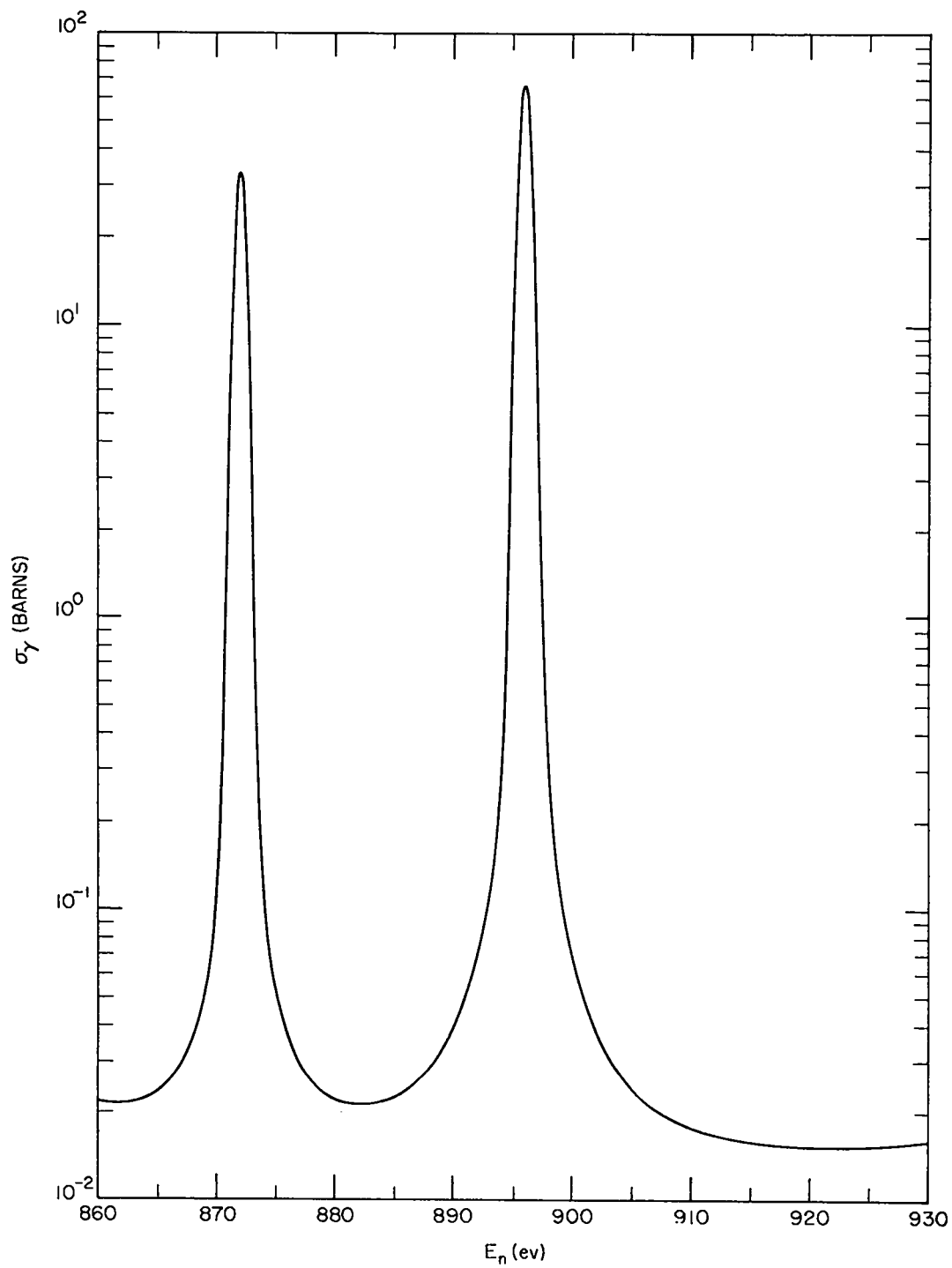
Fig. 17 Thorium-232 radiative capture cross section, \sigma_\gamma , versus neutron energy, E_n , from 860 to 930 ev for \Gamma = 0.0253 ev.
