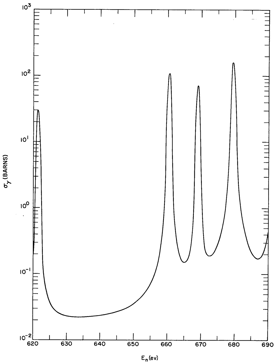
Fig. 13 Thorium-232 radiative capture cross section, \sigma_\gamma , versus neutron energy, E_n , from 620 to 690 ev for T = 0.0253 ev.
